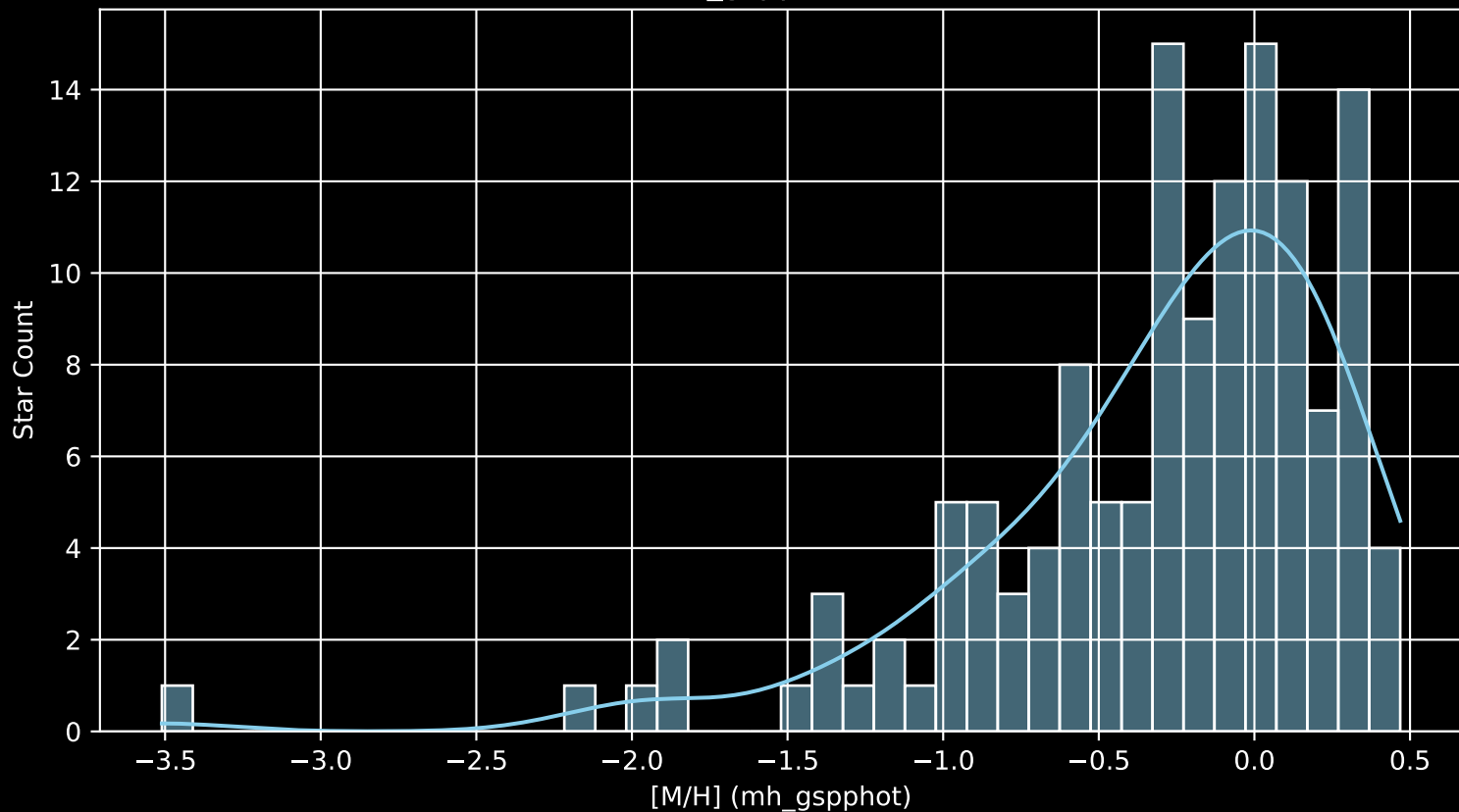
APOGEE DR17 Field: [351-02-O [M/H] (mh_gspphot) (n= 136)
