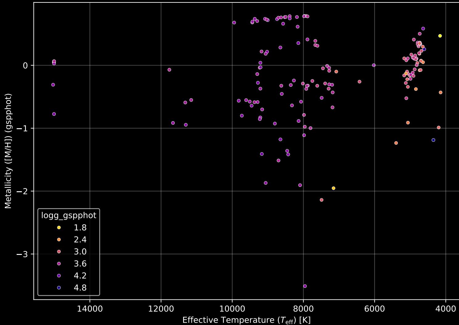
APOGEE DR17 Field: [351-02-O] Stellar Population Parameters (n= 160)
