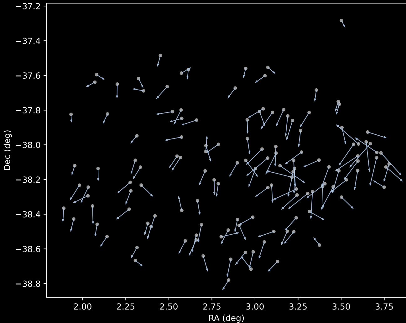
APOGEE DR17 Cluster 1 Proper Motion Vectors (n=131)
