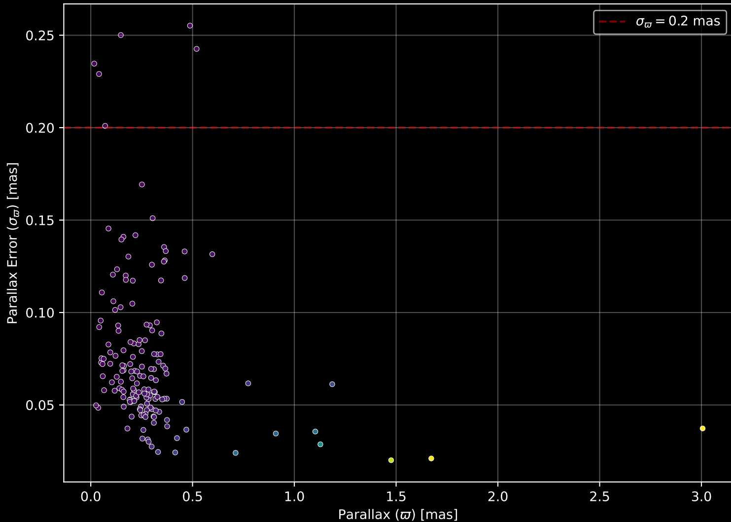
APOGEE DR17 Field: [351-02-O] Parallax Quality (n= 160)
