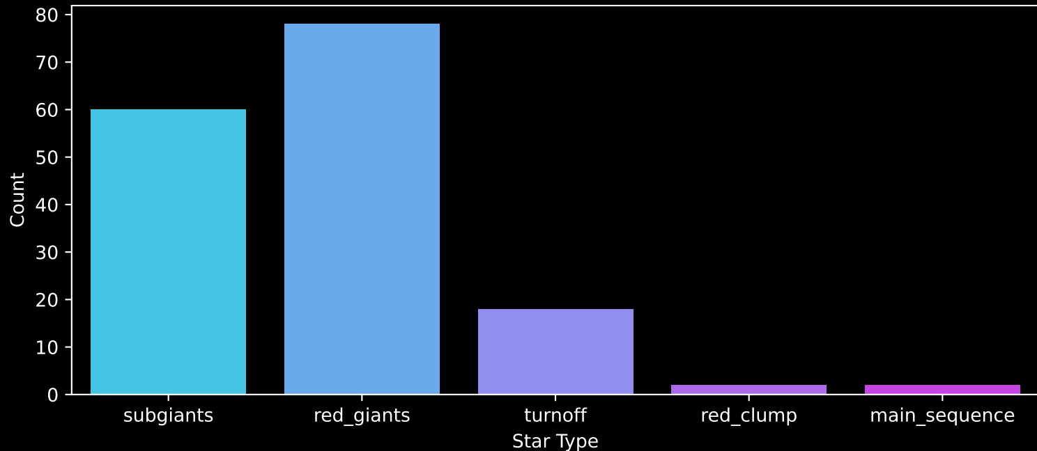
APOGEE DR17 Field: [351-02-O] Count plot of Star Type
