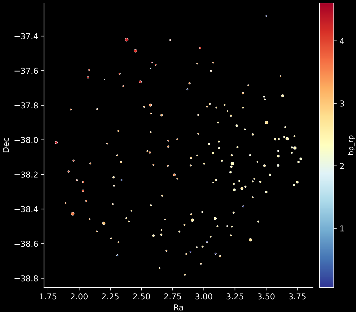
APOGEE DR17 Field: [351-02-O] Stars: 160
