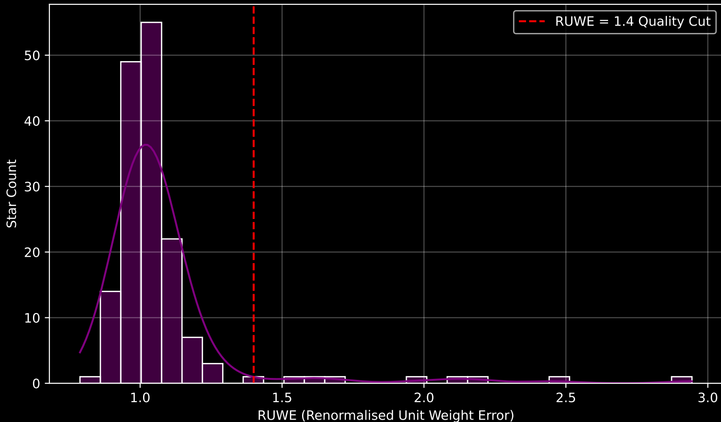
GAPOGEE DR17 Field [351-02-O] RUWE Distribution (n= 160)
