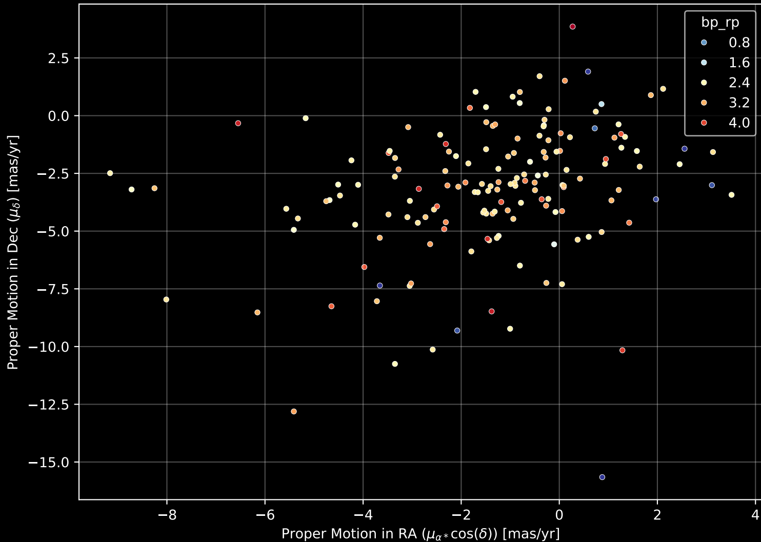
APOGEE DR17 Field: [351-02-O] Proper Motion Diagram (n= 160)
